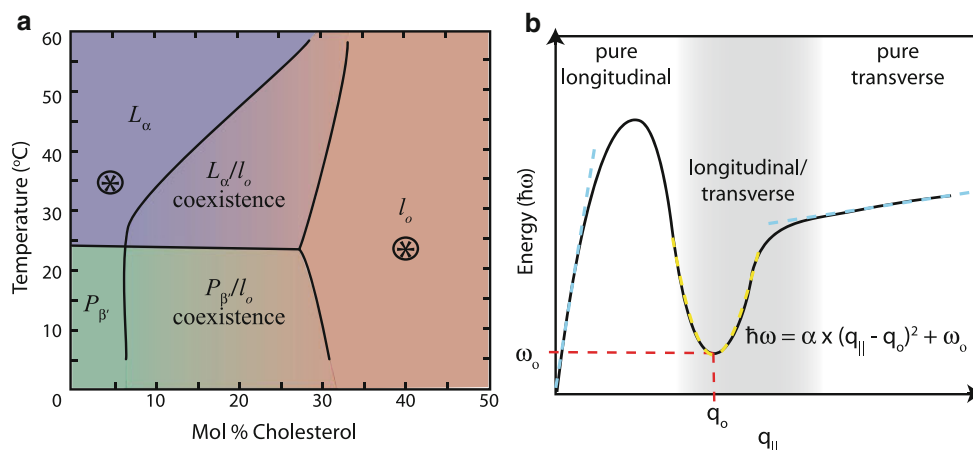
Fig. 2 a Schematic phase diagram of a DMPC cholesterol system as reported by, e.g., Vist 1990; Almeida et al. 1992; Thewalt and Bloom 1992; de Meyer 2009; de Meyer et al. 2010. Besides the well-known gel and fluid phase, the so-called liquid-order phase, is observed at high cholesterol concentrations. The 5 mol% cholesterol sample is in the L_\alpha phase, while the 40 mol% sample is clearly in the l_o phase, as depicted by the \otimes . b A typical lateral dispersion curve observed in
