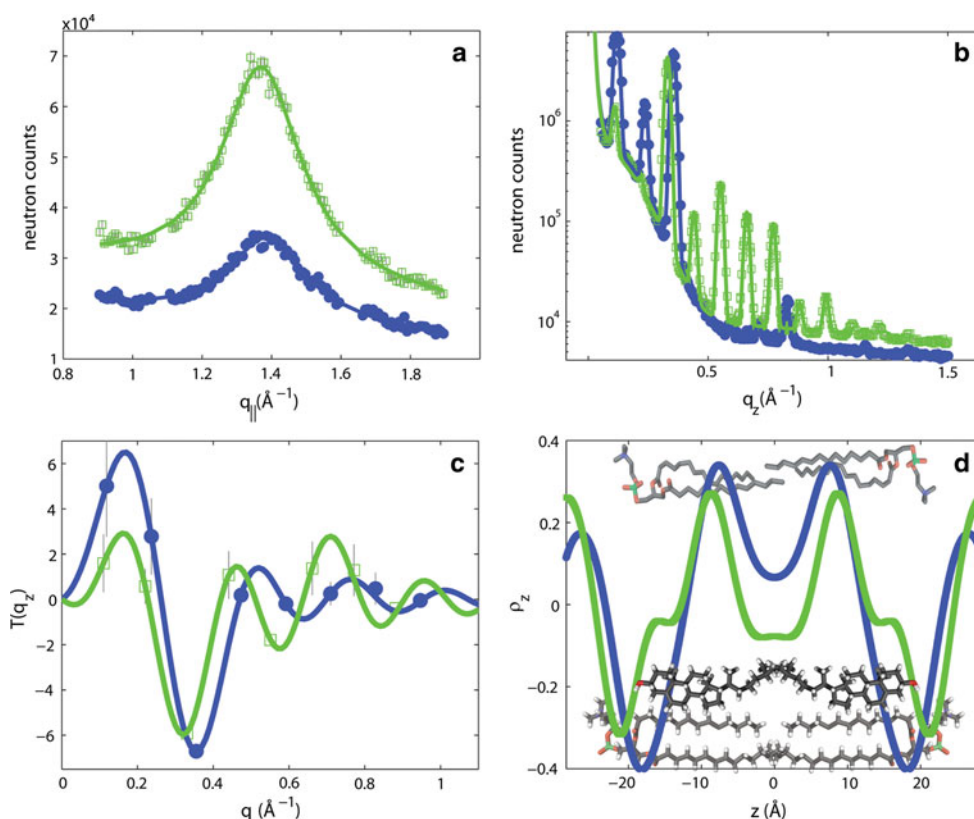
Fig. 4 Overview of the diffraction data: the blue solid lines and data points correspond to the 5 mol% cholesterol sample, while the green solid lines and data points refer to the 40 mol% cholesterol sample. a In-plane scattering ( q_{||} ) used to measure the acyl chain-chain positional correlation peak. Two spurious Bragg peaks from the humidity chamber at \sim 1.1 \text{ Å}^{-1} and \sim 1.65 \text{ Å}^{-1} were omitted from the scans. The solid lines are the Lorentzian fits to the experimental data. b Out-of-plane scattering ( q_z ) and the observation of several Bragg peaks. The position and area of each Bragg peak was determined through the fitting of a Gaussian, including the q^{-4}
