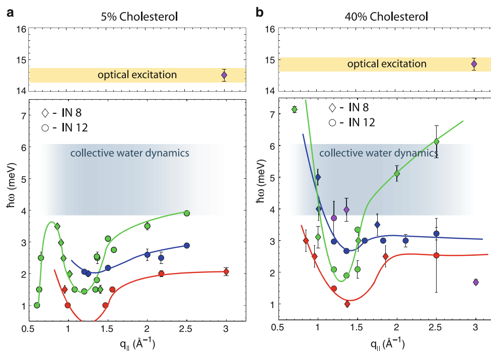
Fig. 6 Energy dispersion curves for DMPC bilayers with a 5 mol% cholesterol and b 40 mol% cholesterol. The dispersion curve corresponding to the gel phase is shown in green and the fluid phase in blue. The liquid-ordered phase, arising from the high concentration of cholesterol in the sample, is depicted by the red curve. The blue band at \sim 4 –6 meV represents the region where excitations due to hydrating water are observed (Paciaroni et al. 2008). The yellow band represents an optical excitation at 14–15 meV, which was predicted by MD simulations (Tarek et al. 2001)
