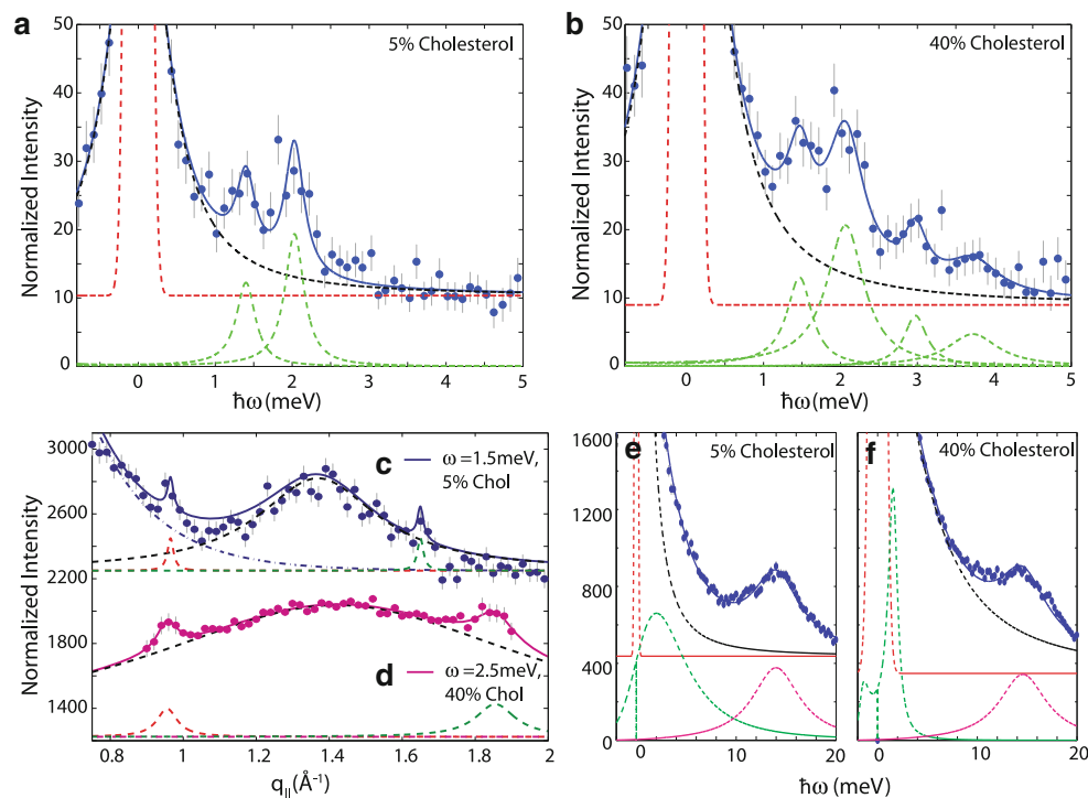
Fig. 5 Overview of the inelastic data: constant- q_{\parallel} scan at q_{\parallel} = 1.2 \text{ \AA}^{-1} . The instrumental resolution is fit with a Gaussian (red), and the relaxation dynamics by a Lorentzian (black) function. The satellite excitations peaks are fit with damped harmonic oscillators (green), with the total fit shown in blue. a Data of 5 mol% and b 40 mol% cholesterol concentration samples. Constant-energy scan showing peaks fitted with Lorentzian curves: c 5 mol% cholesterol at \hbar\omega = 1.5 \text{ meV} . The Lorentzian fits are depicted by dashed black, red and green curves, with an exponential used to fit the background (dashed blue). The total fit is shown as a solid blue line. d 40 mol% cholesterol at \hbar\omega = 2.5 \text{ meV} . The
