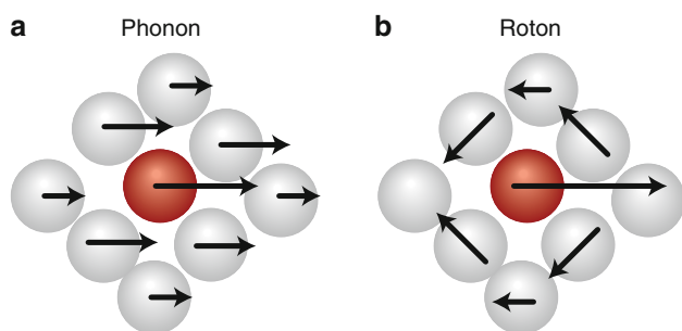
Fig. 7 a Molecular dynamics of particles participating in the propagating sound-like wave, i.e., the longitudinal phonon at small q_{\parallel} -values (long length scales) and b in the “roton” at q_{\parallel} -values in the dispersion minimum. These dynamics are expected to show a mixed, longitudinal and transverse character as neighboring particles couple strongly. Figure adapted from Annett (2004)
