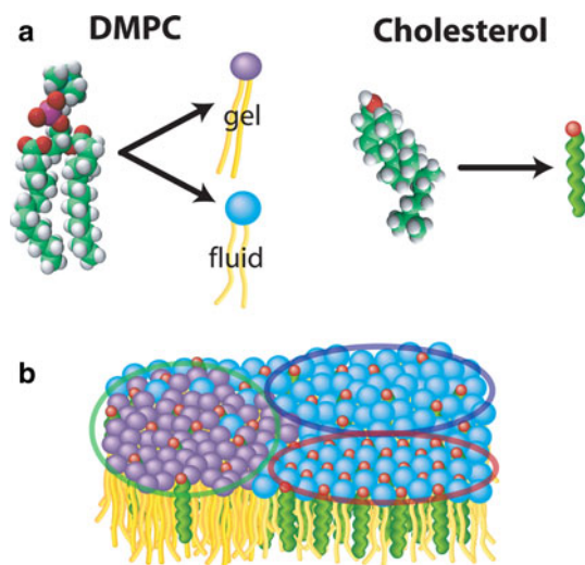
Fig. 1 a Schematic representations of DMPC and cholesterol molecules. In the gel phase, the lipids tails are in the all-trans configuration. At the main transition temperature lipid hydrocarbon tails “melt”, resulting in fluid phase bilayers. b Schematic model of the possible phases present in DMPC/cholesterol systems. The gel, fluid and liquid-ordered phases are highlighted by the green, blue and red circles, respectively
