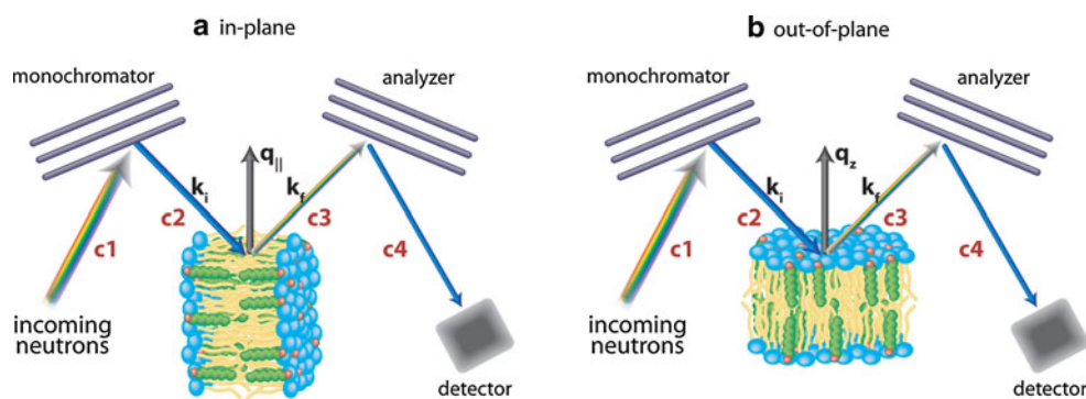
Fig. 3 Schematic representation of a triple axis spectrometer geometry. a Orientation of the sample for in-plane scans such that \mathbf{Q} is in the plane of the membrane ( q_{\parallel} ). b Orientation of the sample for out-of-plane scans such that \mathbf{Q} is perpendicular to the plane of the
